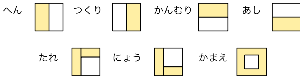
Figure 1: Kanji Radical
